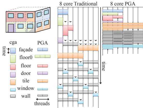
Figure 5: Comparison between a traditional GPU implementation of CGA shape and PGA, which uses multiple threads per rule.. A very simple building is specified by seven rules (left). The traditional implementation frequently leaves most SIMD units unoccupied (center) and is ridden by divergence (black chevrons). The need to flush and read back shapes from global memory introduces additional idle time for the whole GPU. With parallel rule evaluation and rule grouping, PGA can execute much more efficiently on SIMD units (right). Divergence and slow global memory access are avoided. Note that the same amount of work (colored area) is done in both cases, but PGA achieves more efficient scheduling.
