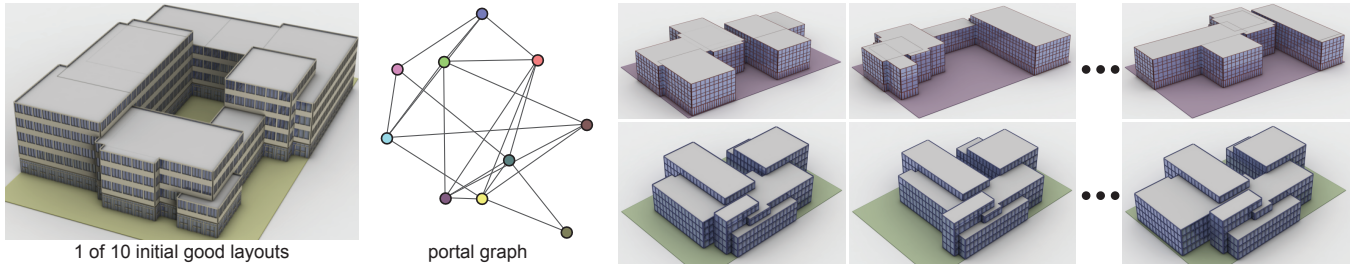
Figure 1: Starting from a set of hard constraints (e.g., regulatory guidelines) and soft constraints (e.g., quality measures), we formulate a constrained optimization to characterize good building layouts. Then, starting from a discrete set of samples of good layouts, we analytically construct local shape spaces around each discrete layout, and link the local shape spaces via a portal graph. Exploration using the portal graph then reveals a family of layout solutions. Importantly, the user is exposed to only good layouts, simplifying layout exploration.
